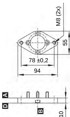
Mounting flange
